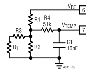
Figure 5. External NTC Thermistor Network
