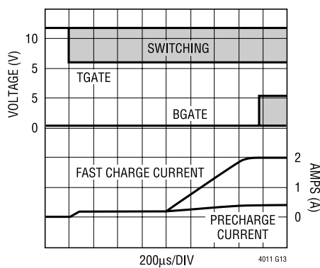
Charger Soft-Start
