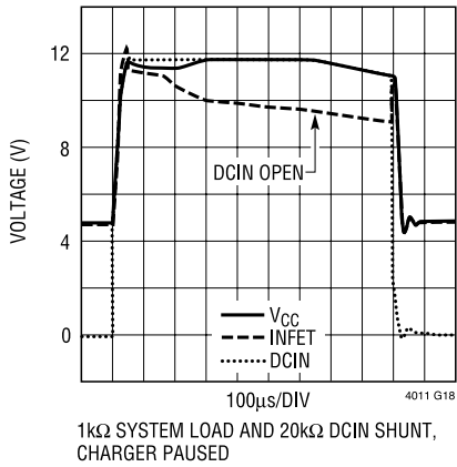
PowerPath Switching
